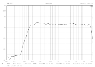
Frequency response
